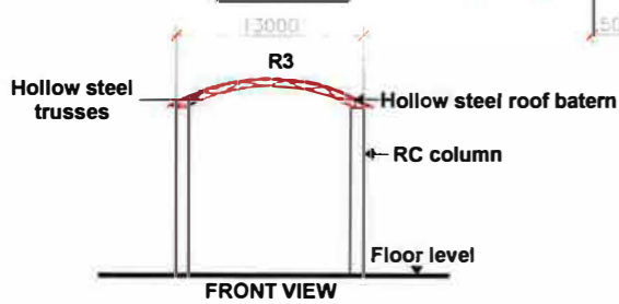
R3 Detail
