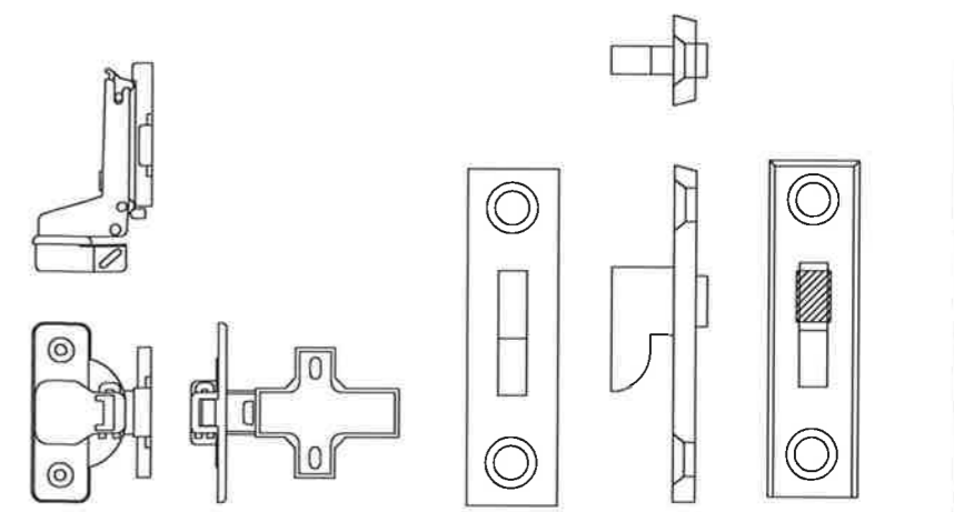
DETAIL 1 4 set Stainless steel safety door hydraulic hinge soft close to manuf's detail
