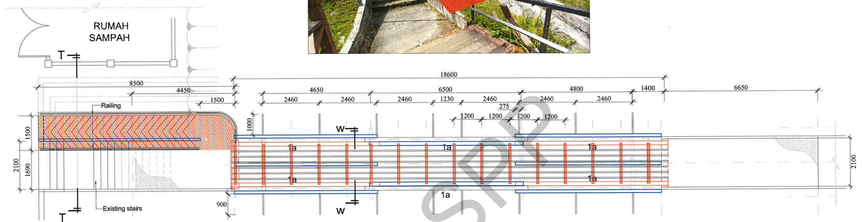
PLAN ( structure ) (JAMBATAN ARKED CENGAL)
