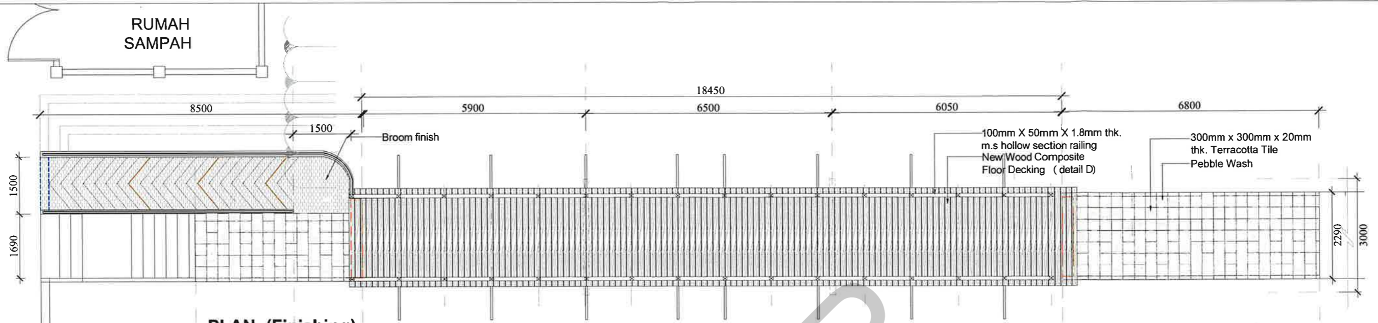
PLAN (Finishing) (JAMBATAN ARKED CENGAL)
