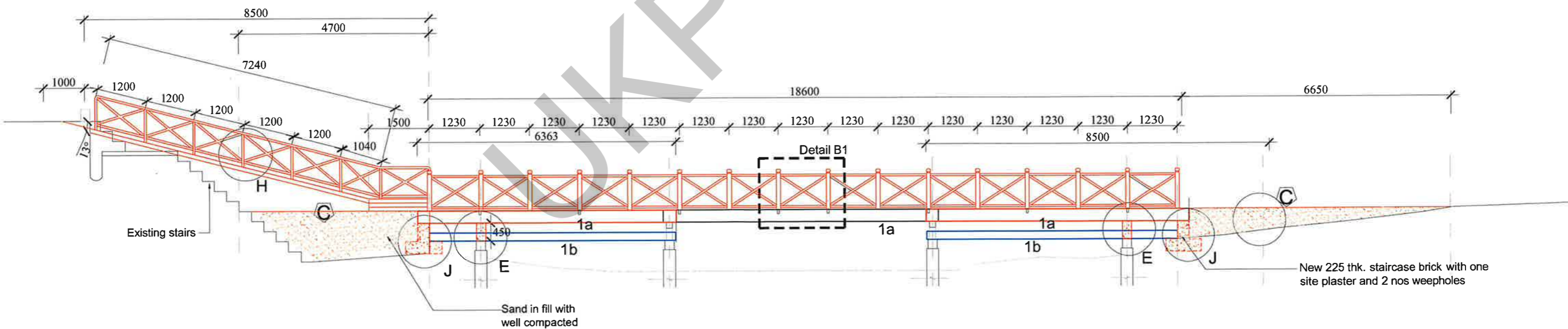
SIDE ELEVATION
