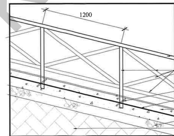
DETAIL H not to scale
