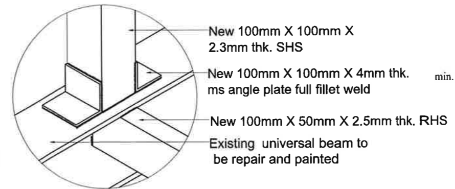
DETAIL A not to scale
