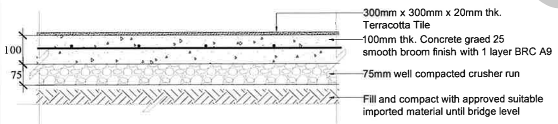
DETAIL C not to scale
