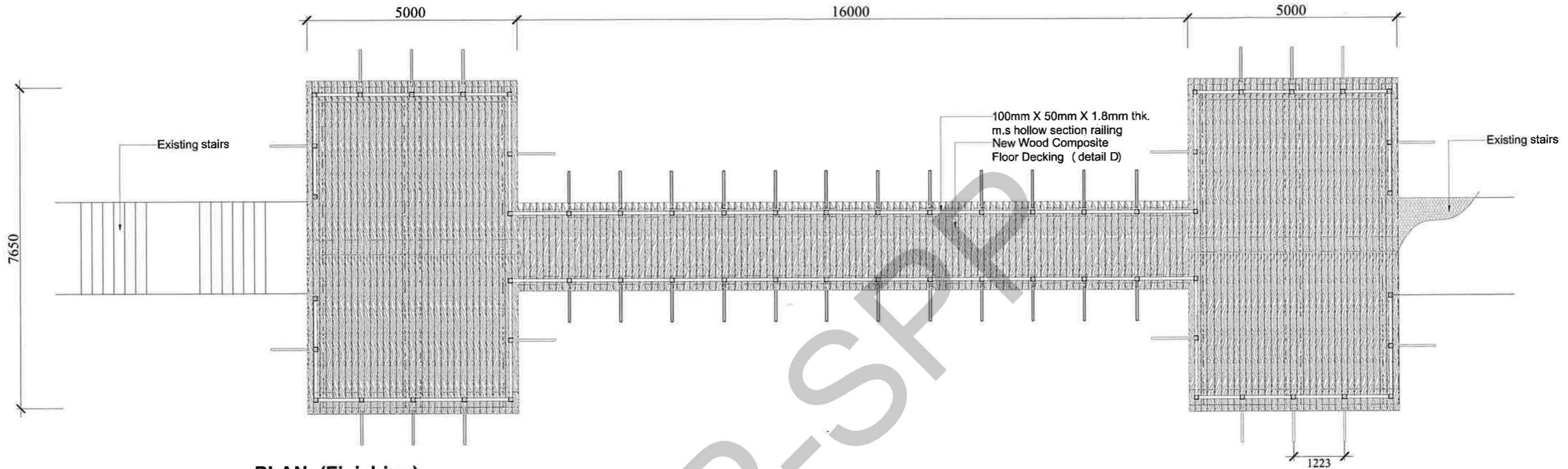
PLAN (Finishing) (JAMBATAN M46) Scale = 1 : 100
