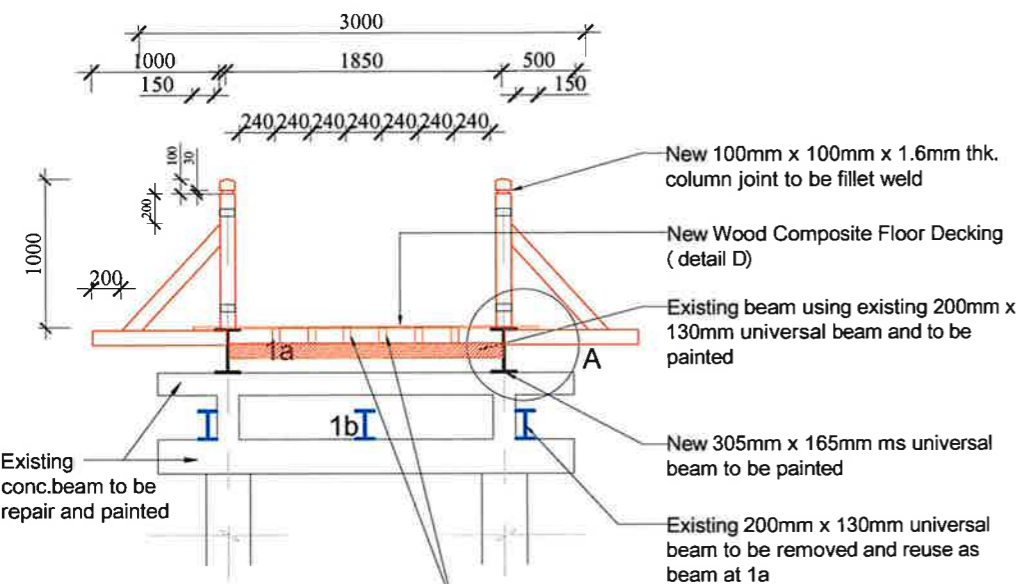
SECTION W - W Scale = 1 : 50
