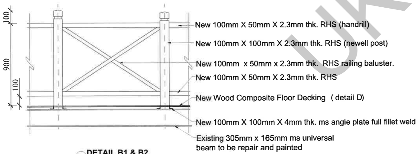
DETAIL B1 & B2 not to scale
