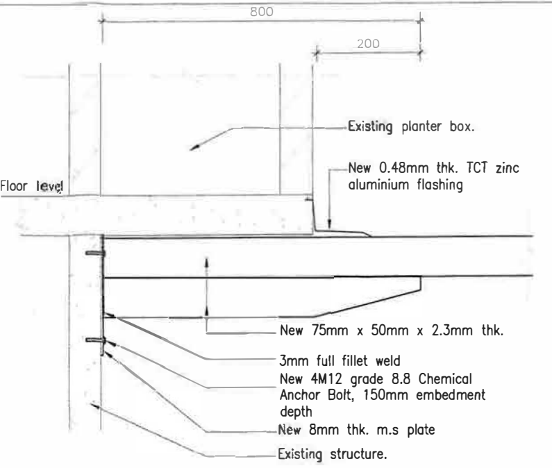
TYPICAL DETAIL 1
