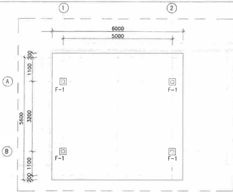
FOUNDATION PLAN
