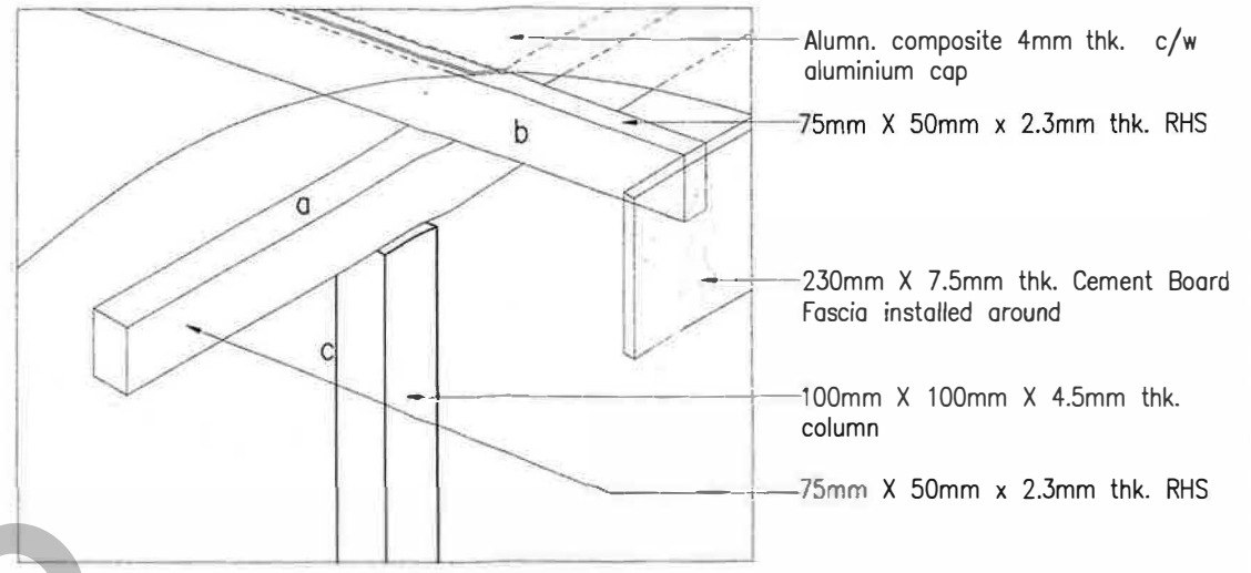
ISOMETRIC VIEW DETAIL A
