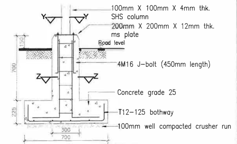
DETAIL F-1
