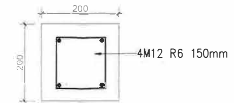
SECTION Z - Z
